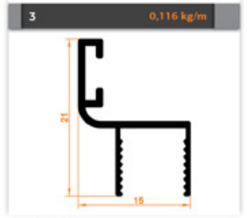
Küçük H Fitil Small H Wick
