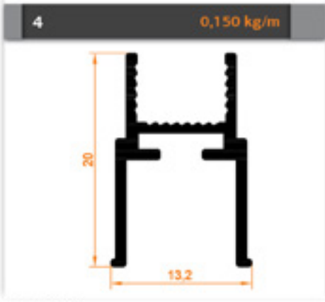
Orta H Fitil Middle H Wick
