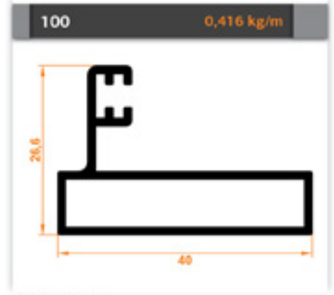
Dar Yan Dikme Thin Side Column
