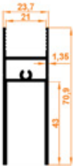
Isicam Baza Double Glass Base Profile
