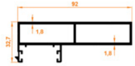
3'lü Yan Kasa Triple Side Case Profile
