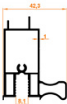
Tek Cam Birleştirme Kilit Profili Single Glass Combination Lock Profile
