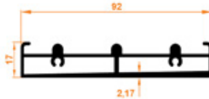
3'lü Alt Kasa Triple Bottom Case Profile
