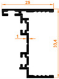
Sabit Cam Menteşe Profili Constant Glass Hinge Profile
