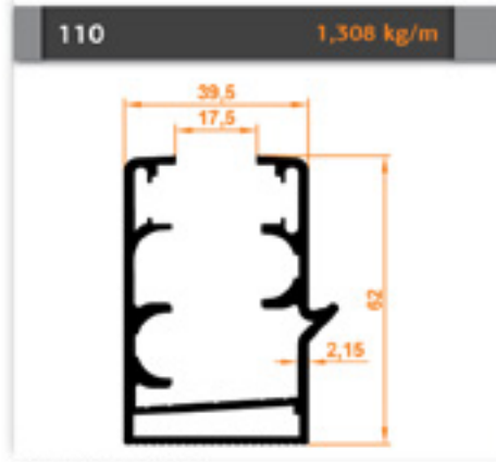
Oluklu Kasa Profili Corrugated Case Profile
