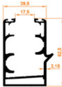
Oluklu Düz Kasa Fitilli Profili Flat Corrugated Case with Weather Stripe Profile
