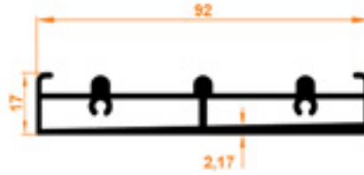
3'lü Alt Kasa Triple Bottom Case Profile
